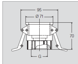
Quick-fit pipe connection (female thread)
